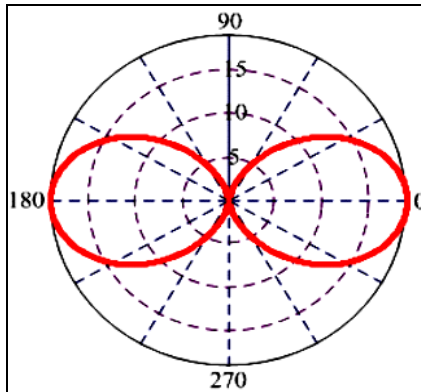
Fig. 3: Dipole antenna radiation pattern.
