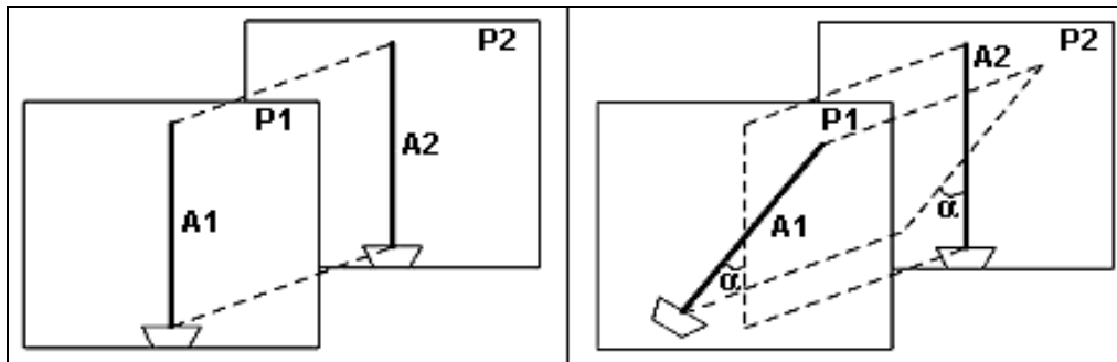
Fig. 2: Inclination of AIS dipole Antenna – courtesy of manual: by Ilcev [4]
