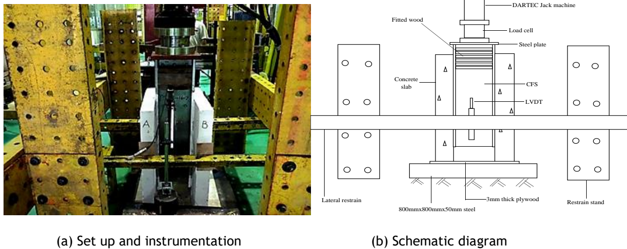
Fig. 2: Push-out test arrangement
